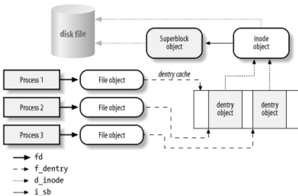
Figure 12-2. Interaction between processes and VFS objects
